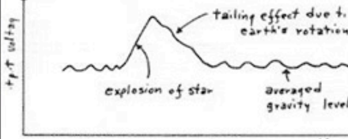
(a) Typical Nova Response
