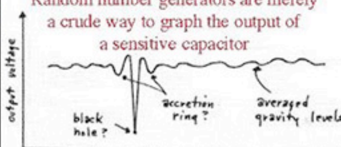
(c) Typical Black Hole Response
