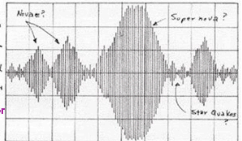
(a) Typical Nova Response
