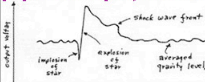
(b) Typical Supernova Response
