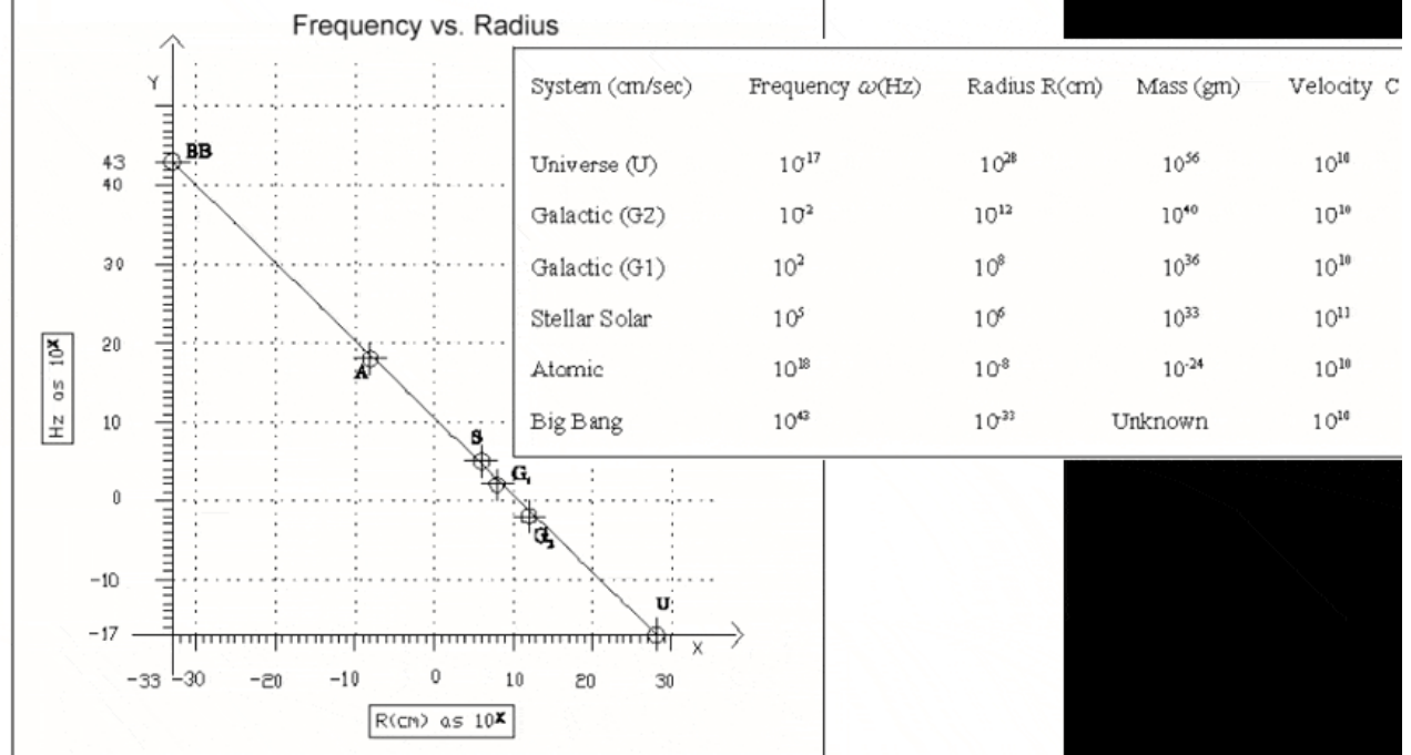
Figure 2a. A scaling law for organized matter of frequency vs. radius. The black hole system is presented in this figure. Plotted from the top left is the mini black hole at the Planck distance of 10^{-33} \text{ cm} through to the stellar-sized black holes, larger black holes, galactic center black holes and at the lower right is a Universe-sized black hole. Note that in between the stellar size and the Planck distance mini black hole we have included a data point for the atomic size which we as well calculate a new value for its mass that includes the energy available in the vacuum space of a nuclei and yields the correct radius to describe an atomic resolution as mini black holes (see equation (5) to (18)). It is of interest that the microtubules of eukaryotic cells, which have a typical length of 2 \times 10^{-8} \text{ cm} and an estimated vibrational frequency of 10^9 \text{ to } 10^{14} \text{ Hz} lie quite close to the line specified by the scaling law and intermediate between the stellar and atomic scales [19].
