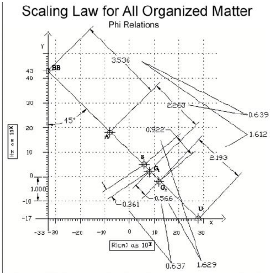
Figure 2b. We note that the distance between the data points on our graph, when divided with each other as in Figure 2b, yields a very close approximation to the familiar \Phi(\phi) ratio given by (1+\sqrt{5})/2 \approx 1.618 and its inverse (1-\sqrt{5})/2 \approx 0.618 . It is both appropriate and significant that the so called “golden ratio” is reflected in our scaling law (which maps energy dynamics at all scales), since it is prominently found everywhere in nature and has marked the evolution of cosmological mechanics and modern physics [18], from Kepler’s solar system modeling [20] to aperiodic Penrose tilings [21], including recent work on the thermodynamic phase transition of black holes showing a change of state from negative specific heat to positive specific heat at (1-\sqrt{5})/2 \approx 0.618 [22].
